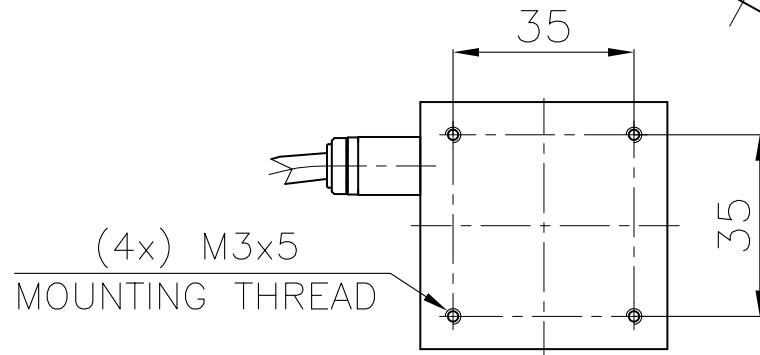
VIEW A
